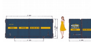
10m3 Absetzcontainer (380x180x150)
