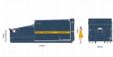
Abroll-Presscontainer 20-25m3
