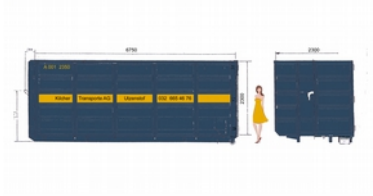
36m3 Abrollcontainer offen
